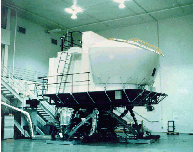
Offense Station Mission Trainer (OSMT)
